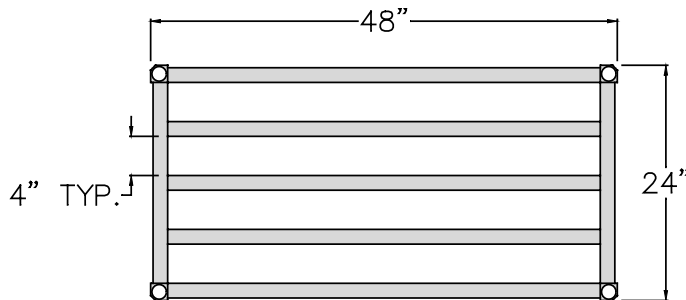
#2448HD Shelf
