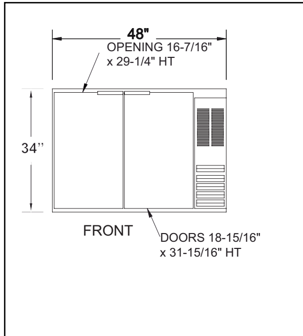
VBB-48
